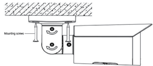
Figure 2-2 Fixed camera
